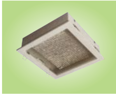
DLL2202 Input voltage: AC90-260V Power: 22W Size: 300*300mm Color temperature: 5000-6000K Protection Class: IP60
