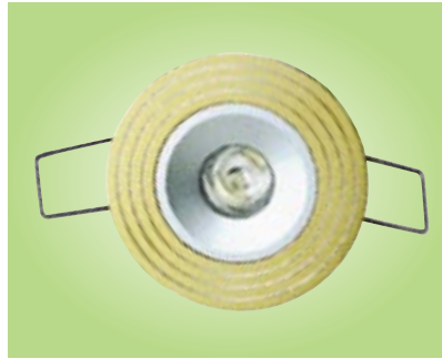
DLL2011 Input voltage: AC110V-240V Size: 63*26mm/1*1W Cut-out: 44mm Beam angle: 8/15/30/45 Material: Aluminum profiles precision work
