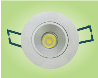
DLL2010 Input voltage: AC110V-240V Size: 63*26mm/1*1W Cut-out: 44mm Beam angle: 8/15/30/45 Material: Aluminum profiles precision work
