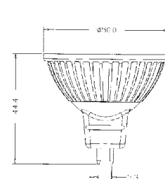
GU5.3
