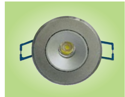
DLL2015 Input voltage: AC110V-240V Size: 70*36mm/1*3W Cut-out: 55mm Beam angle: 8/15/30/45 Material: Aluminum profiles precision work
