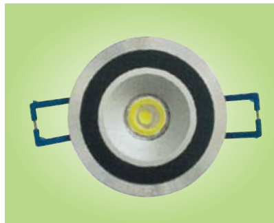
DLL2014 Input voltage: AC110V-240V Size: 63*26mm/1*1W Cut-out: 44mm Beam angle: 8/15/30/45 Material: Aluminum profiles precision work
