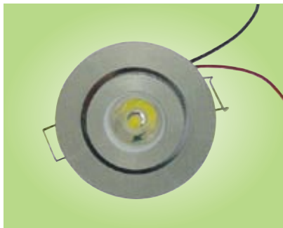
DLL2013 Input voltage: AC110V-240V Size: 53*24mm/1*1W Cut-out: 42mm Beam angle: 8/15/30/45 Material: Aluminum profiles precision work
